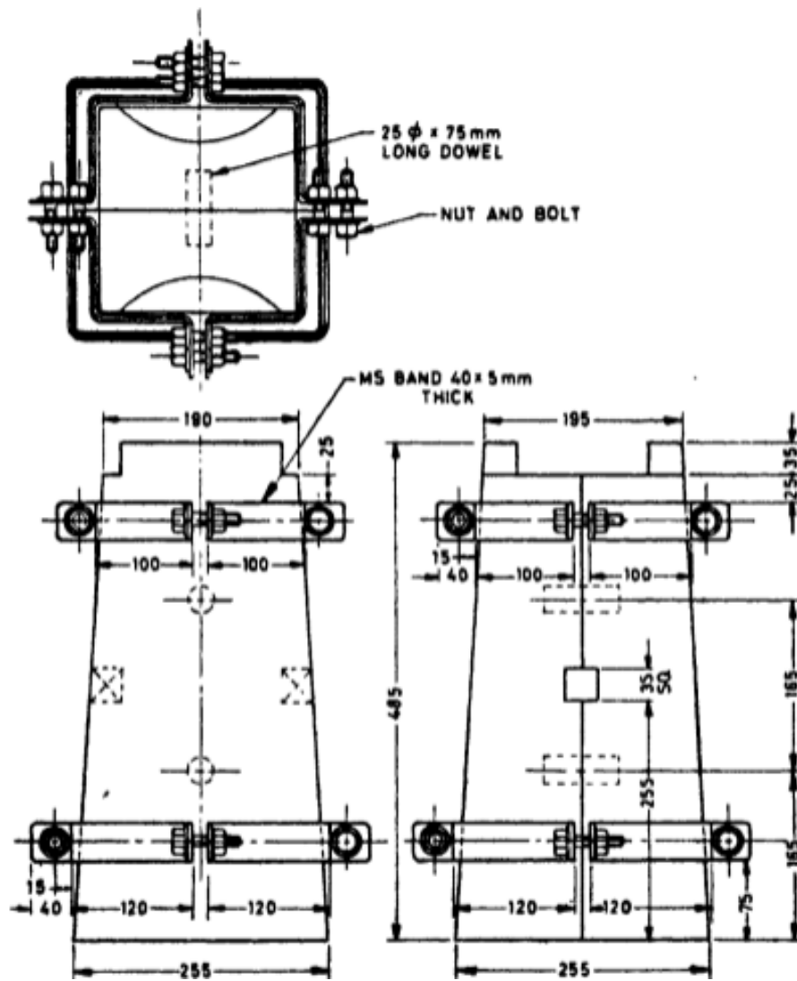
Fig. 2 Anvil Block No. 2 (For 25 kg Anvil)
